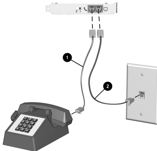
Connecting Your Digital DSL/56K Modem for Use with the 56K ITU V.90 Standard
