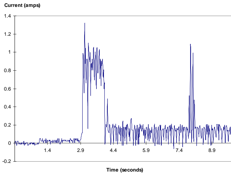
Figure 1. Typical startup and operation current profile
