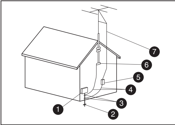
Antenna Grounding
