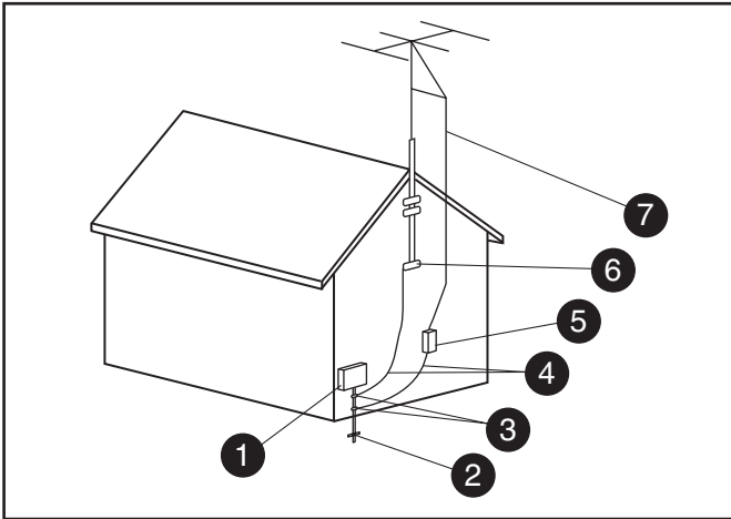
Antenna Grounding
