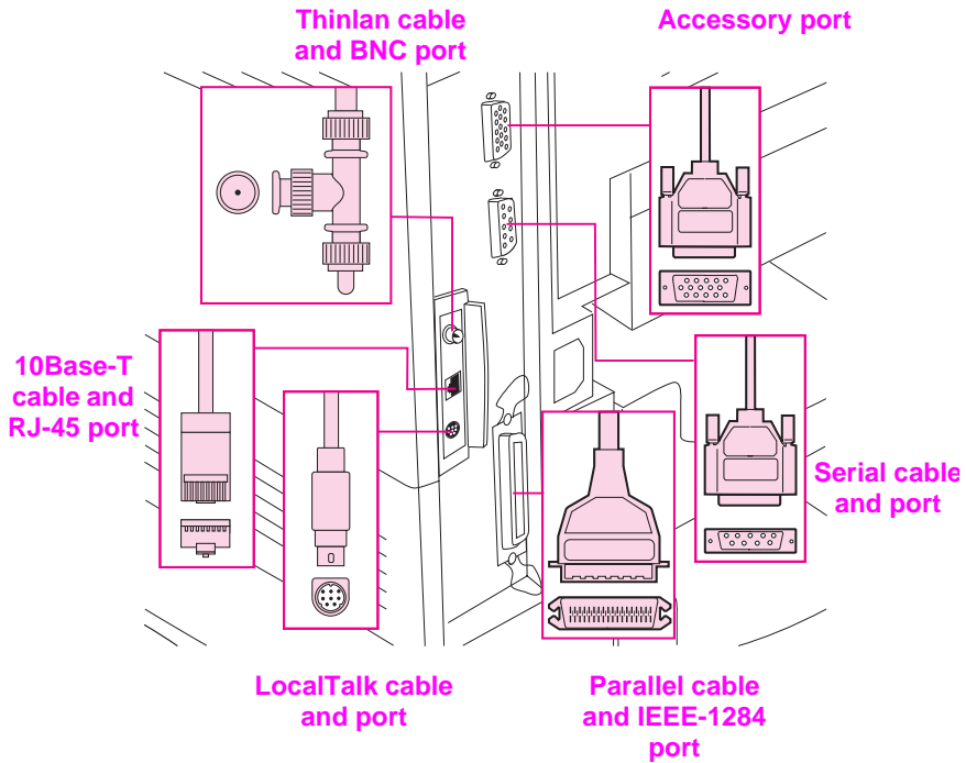
Figure 7 Interface Ports
