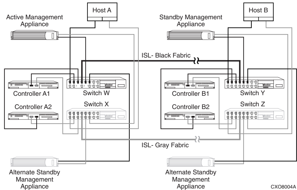
Figure 61: Continuous Access EVA basic configuration
