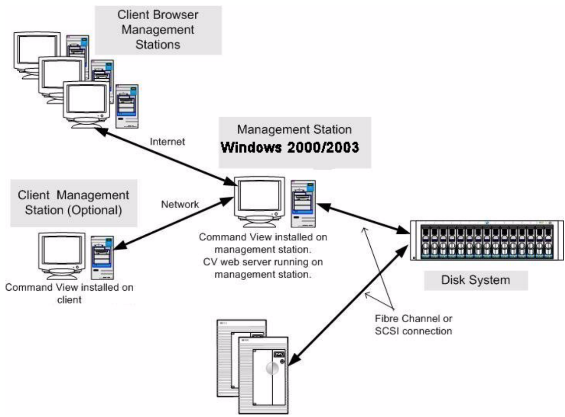
Figure 2 Non- Native Host Management Configuration
