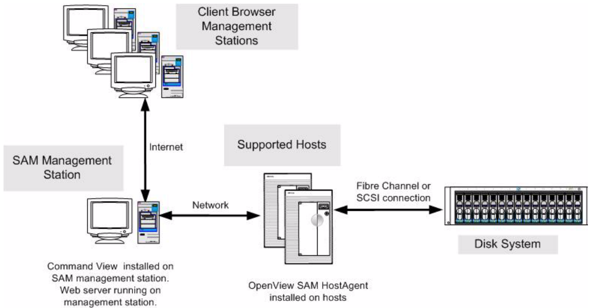
Figure 3 HP OpenView Storage Area Manager Management Configuration
