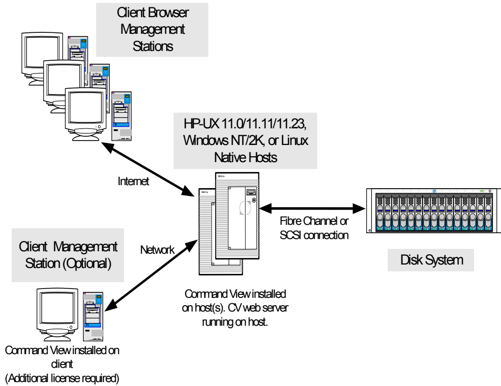
Figure 1 Native Host Management Configuration
