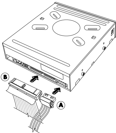
PATA Optical Disc Drive
