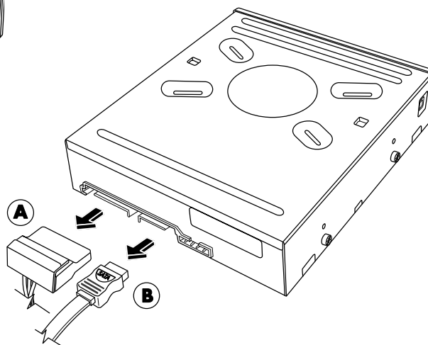
SATA Optical Disc Drive
