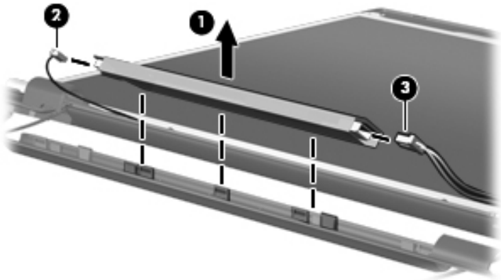
Removing the Display Inverter
