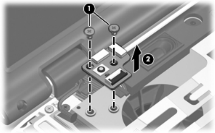
Removing the Power Button Board
