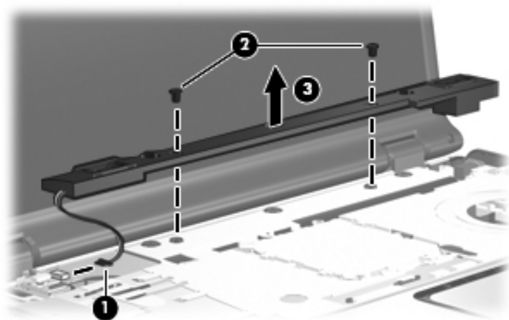
Removing the Speaker Assembly
