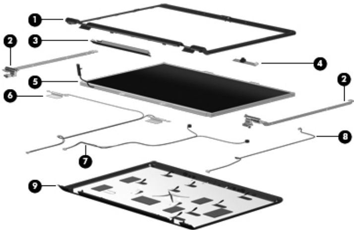
Display Assembly Components
