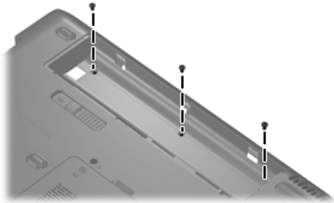
Removing the Switch Cover Screws
