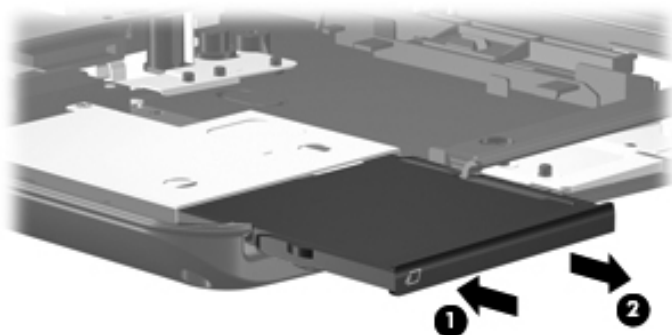
Removing the ExpressCard Slot Bezel
