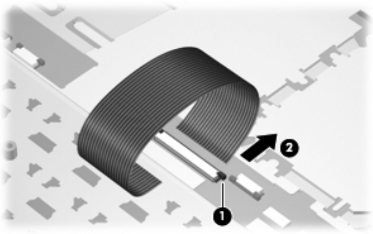
Disconnecting the Keyboard Cable
