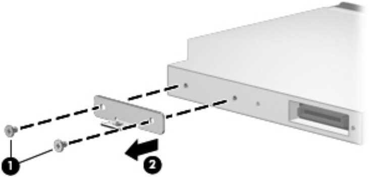
Removing the Optical Drive Bracket
