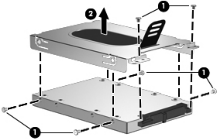
Removing the Hard Drive Frame
