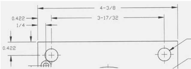
Figure 4-2 CAD drawing scanned at 300 dpi
