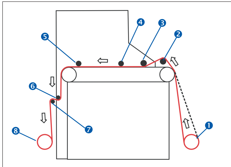
Media route in the takeup system
