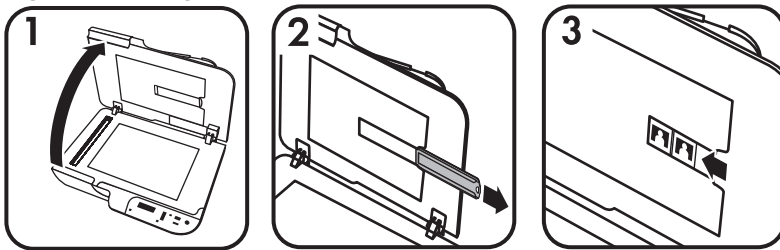
Figure 2-1 Chargement de diapositives
