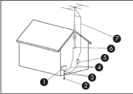
Antenna Grounding
