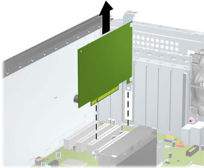
Figure 2-12 Removing a Standard PCI Expansion Card
