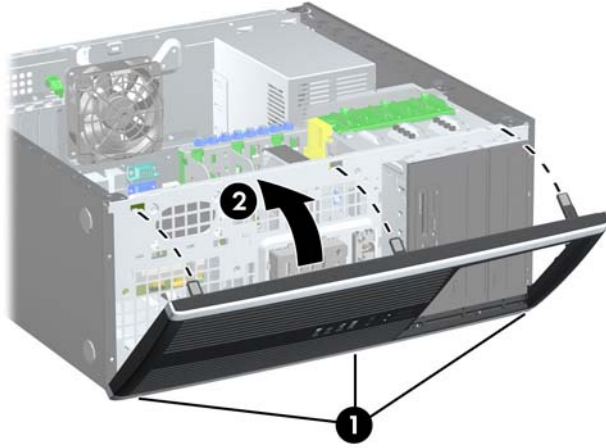
Figure 2-6 Replacing the Front Bezel
