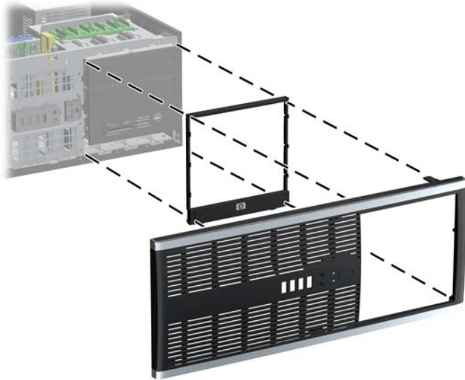
Figure 2-39 Changing from a Minitower to a Desktop Configuration
