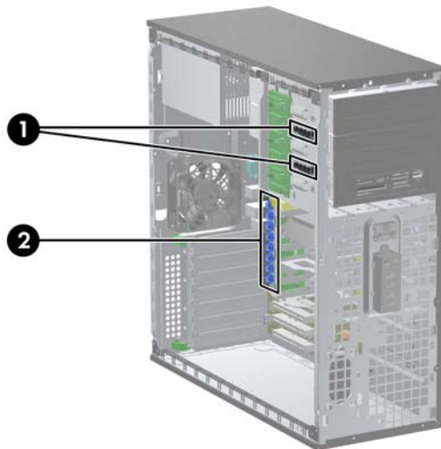
Figure 2-22 Extra Guide Screw Locations
