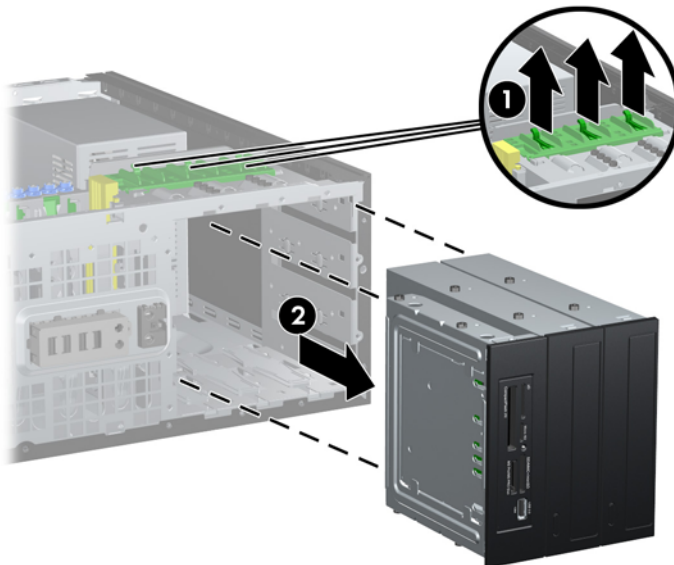
Figure 2-37 Releasing the 5.25-inch Drives from the Drive Bays (Minitower)
