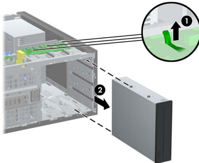
Figure 2-20 Removing a 5.25-inch Drive in the Minitower Configuration (Optical Drive shown)
