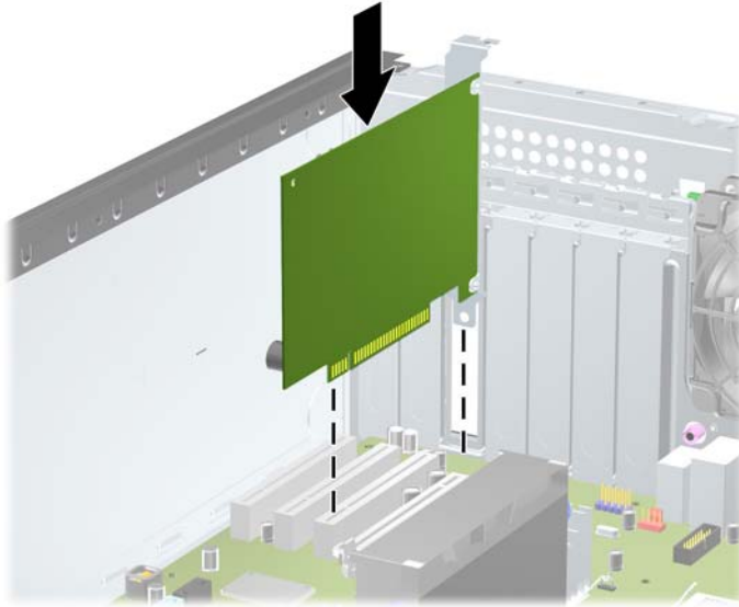
Figure 2-14 Installing an Expansion Card
