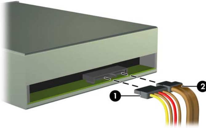
Figure 2-25 Connecting the Drive Cables (Optical Drive shown)
