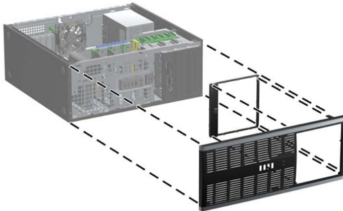
Figure 2-42 Changing from a Desktop to a Minitower Configuration
