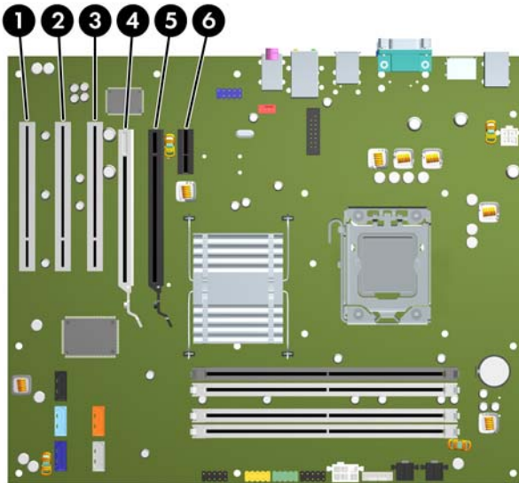
Figure 2-9 Expansion Slot Locations
