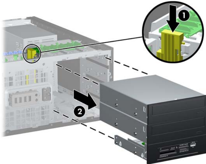
Figure 2-40 Releasing the 5.25-inch Drives from the Drive Bays (Desktop)
