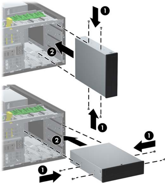
Figure 2-24 Installing a 5.25-Inch Drive in a Minitower (top) and Desktop (bottom)
