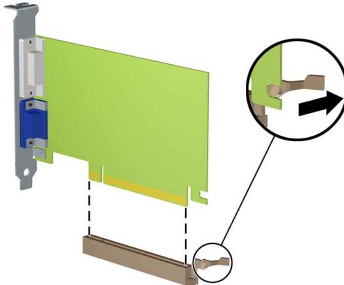
Figure 2-13 Removing a PCI Express x16 Expansion Card
