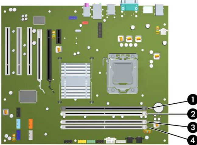
Figure 2-7 DIMM Socket Locations
