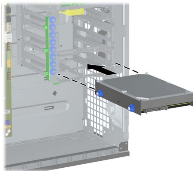
Figure 2-27 Installing a Hard Drive into the Hard Drive Bay
