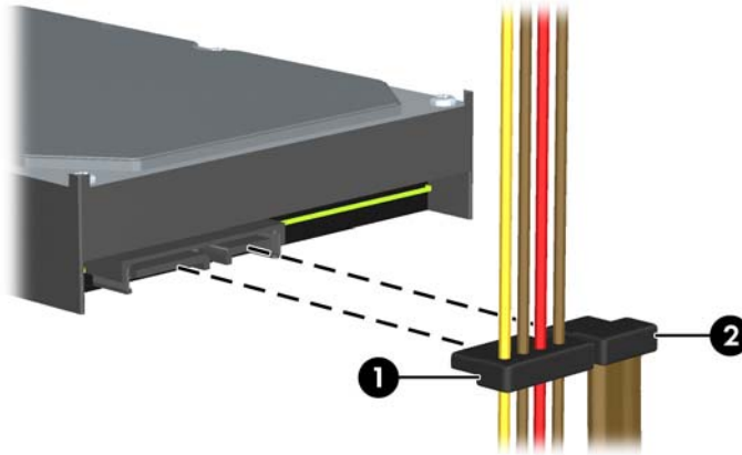
Figure 2-28 Connecting the Power Cable and Data Cable to a SATA Hard Drive
