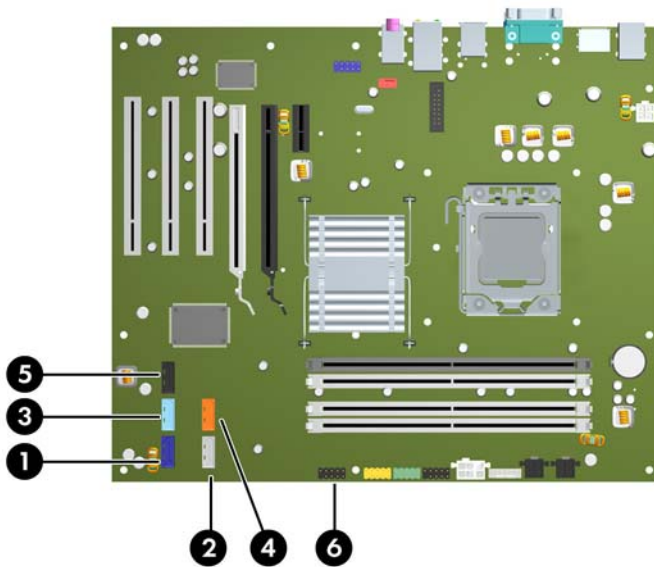
Figure 2-23 System Board Drive Connections
