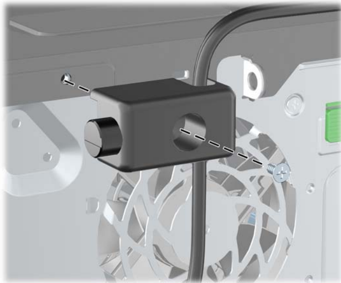
Figure C-5 Attaching the Lock to the Chassis
