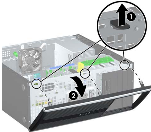
Figure 2-4 Removing the Front Bezel
