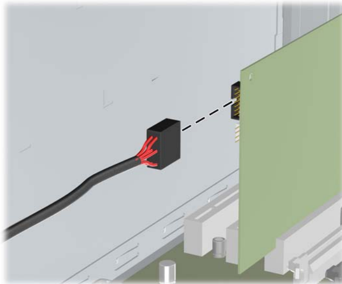
Figure 2-18 Disconnecting the Media Card Reader 1394 Cable
