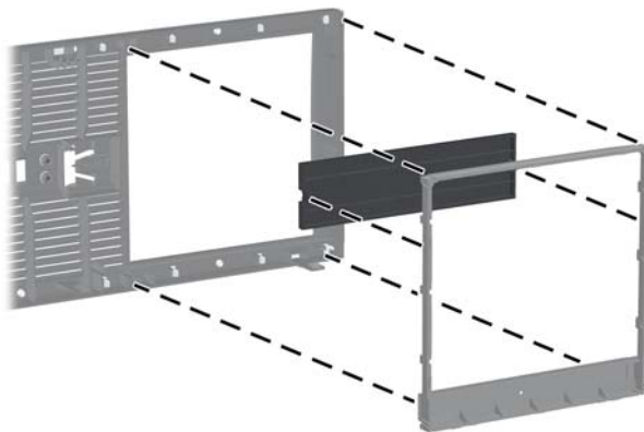
Figure 2-5 Removing Bezel Blanks from the Subpanel (Desktop Shown)
