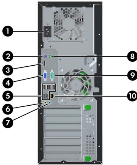
Figure 1-4 Rear Panel Components
