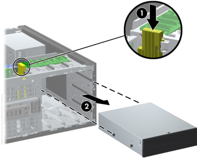
Figure 2-19 Removing a 5.25-inch Drive in the Desktop Configuration (Optical Drive shown)
