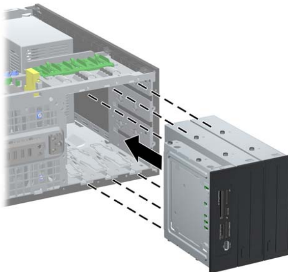
Figure 2-41 Installing a Drive in the Minitower Configuration
