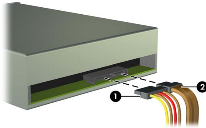
Figure 2-16 Disconnecting the Optical Drive Cables
