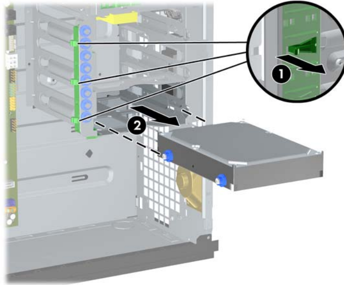
Figure 2-21 Removing a Hard Drive
