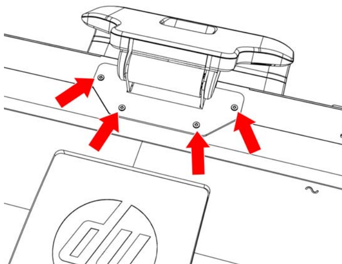
Figure 3-4 Location of screws securing base to monitor
