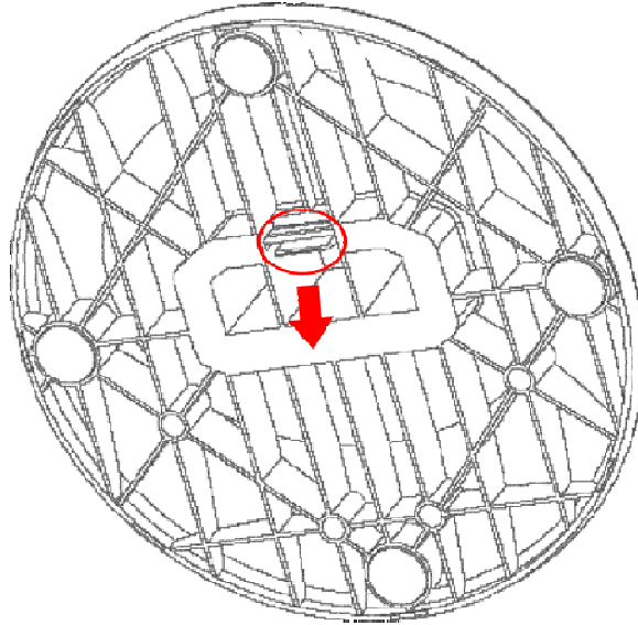
Figure 3-4 Remove the stand from monitor
