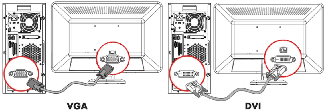
Figure 3-6 Connecting the VGA or a DVI-D (select models) cable
