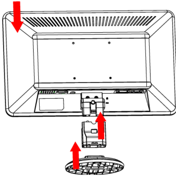
Figure 3-1 Installing the monitor column and stand
