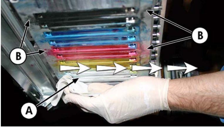
Figure 17 Wiping printheads
