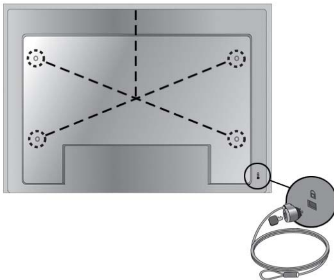
Figure 3-20 Orifices de montage VESA
