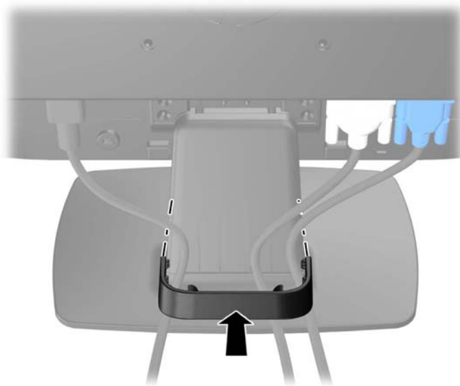
Figure 3-5 Installing the Cable Management Clip
