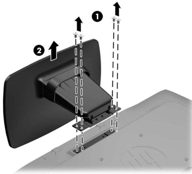
Figure 3-7 Removing the Pedestal Neck Screws
