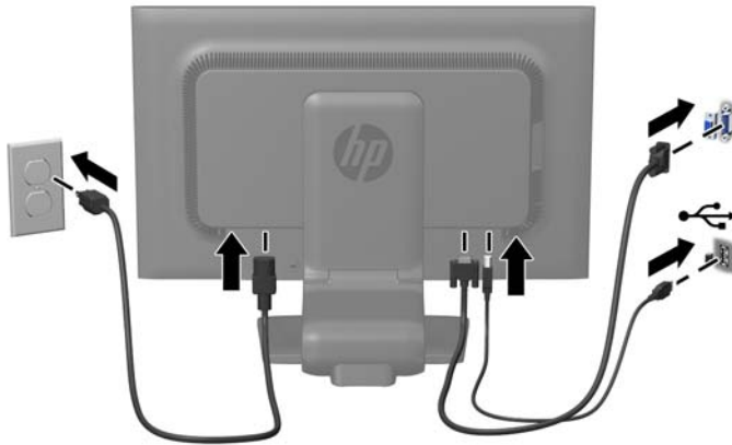
Figure 2-4 Connecting the Cables
