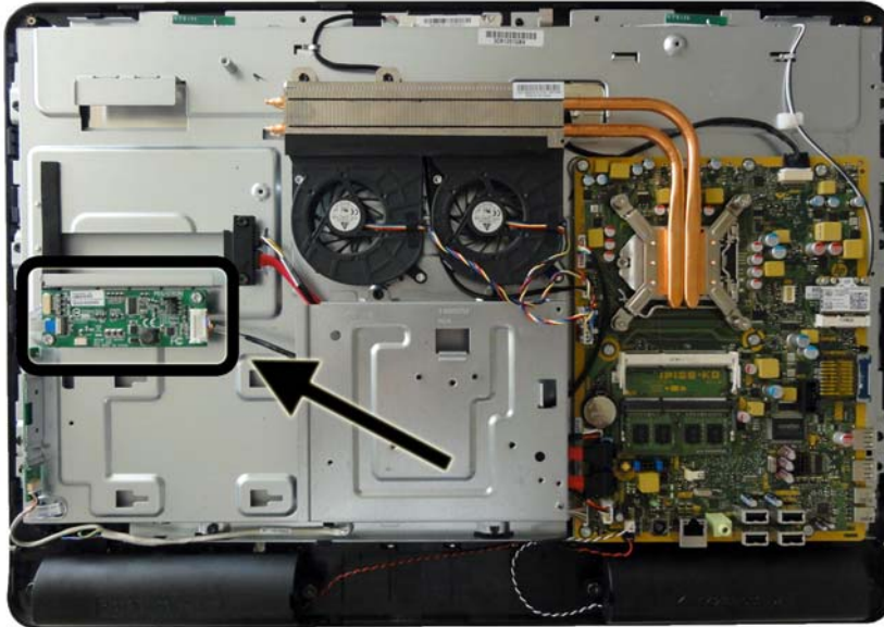
Figure 6-35 Converter board location
