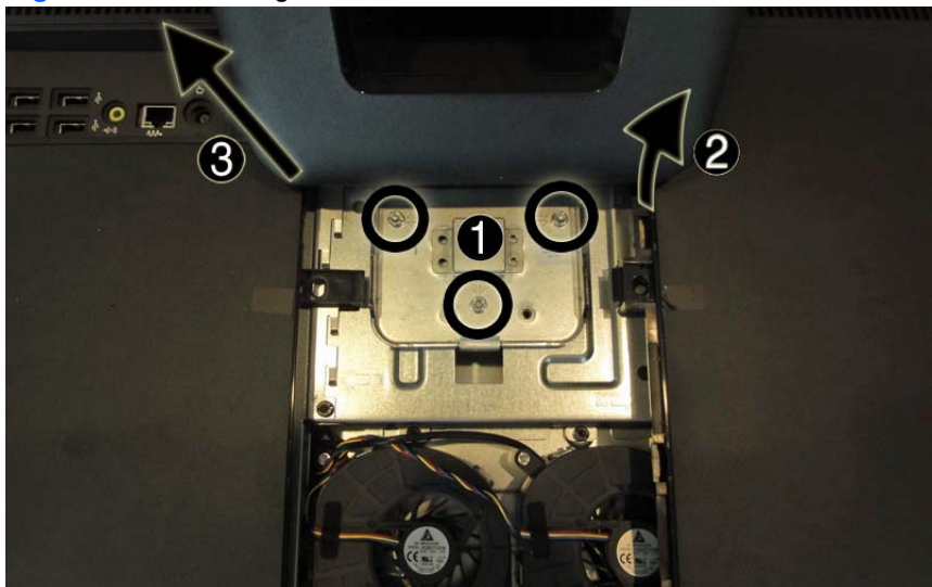
Figure 6-5 Removing the stand
