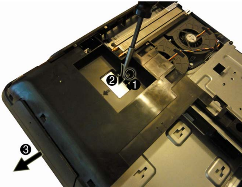
Figure 6-11 Removing the optical drive
