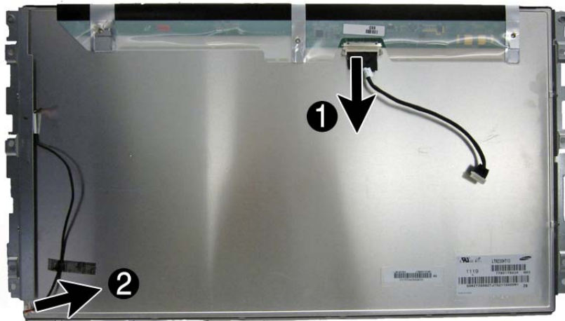
Figure 6-57 Removing the display cable and backlight cables from the display panel (Samsung panel shown)
