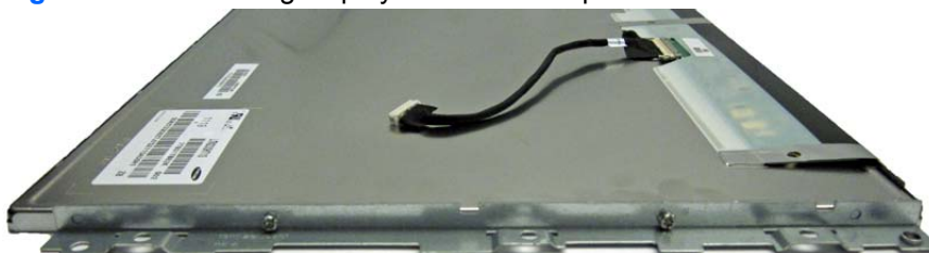
Figure 6-61 Samsung display cable and left panel bracket
