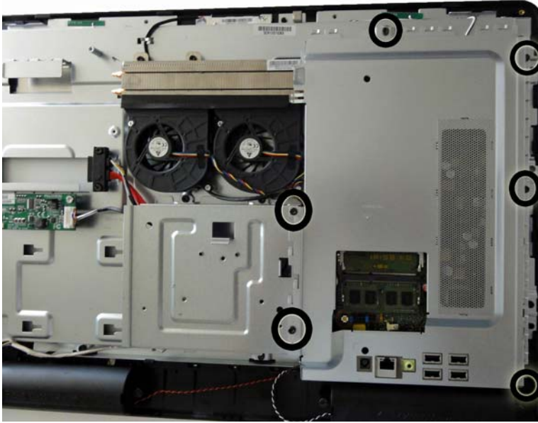
Figure 6-29 Removing the system board cover
