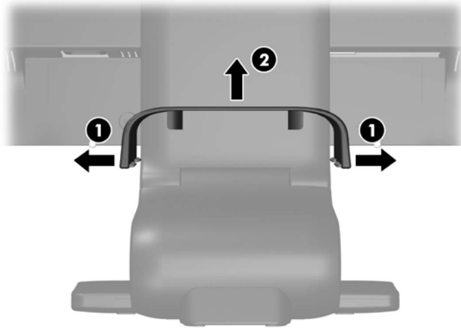
Figure 3-3 Removing the Cable Management Clip
