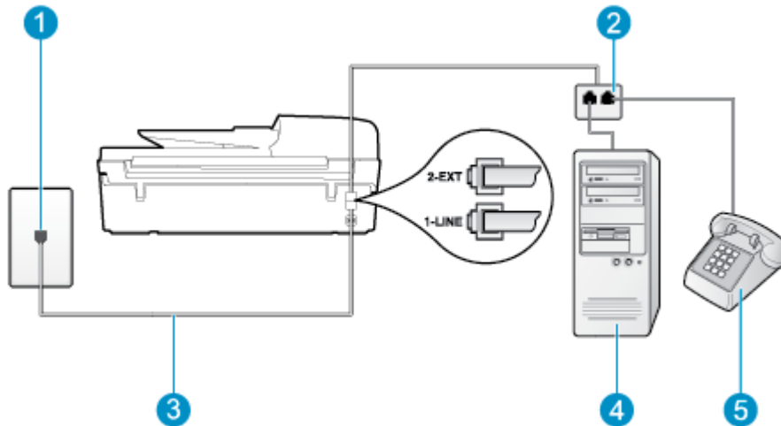
Gambar B-9 Tampak belakang printer
