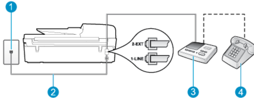
Gambar B-12 Tampak belakang printer
