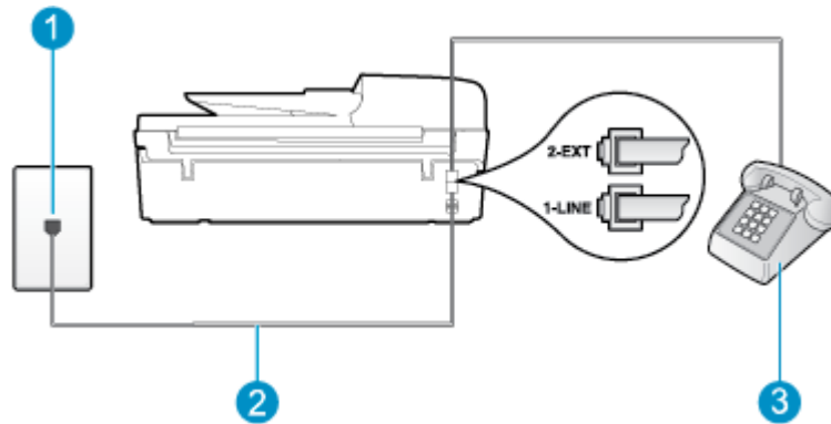
Gambar B-4 Tampak belakang printer
