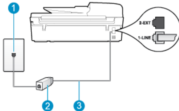
Gambar B-2 Tampak belakang printer
