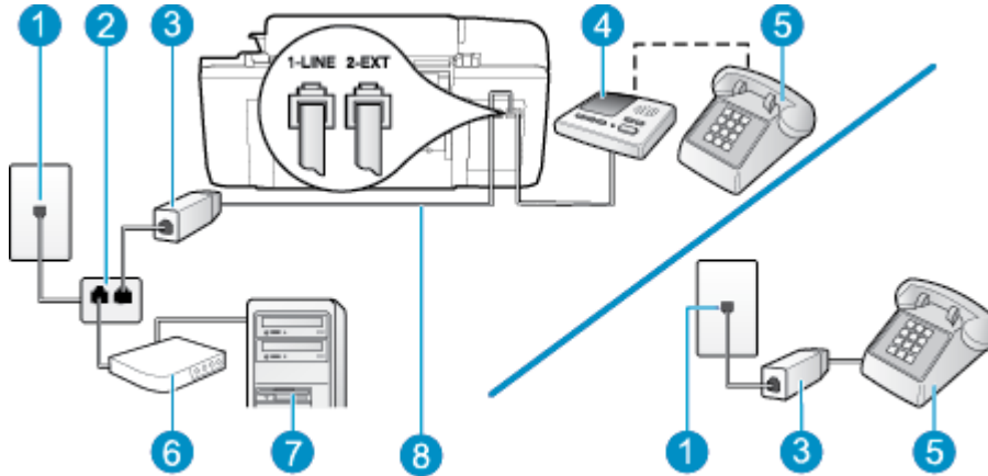
Gambar B-15 Tampilan belakang printer
