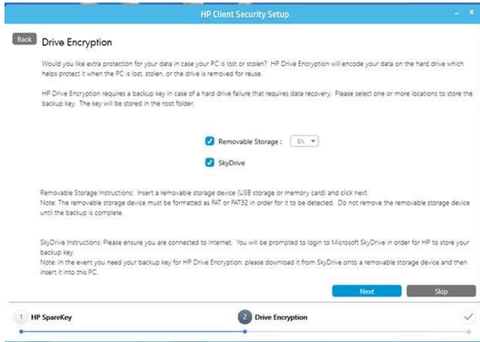
Figure 7 Wizard Page
