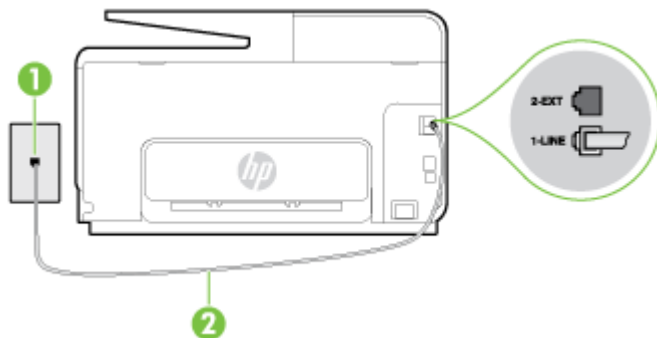
Figure B-3 Back view of the printer
