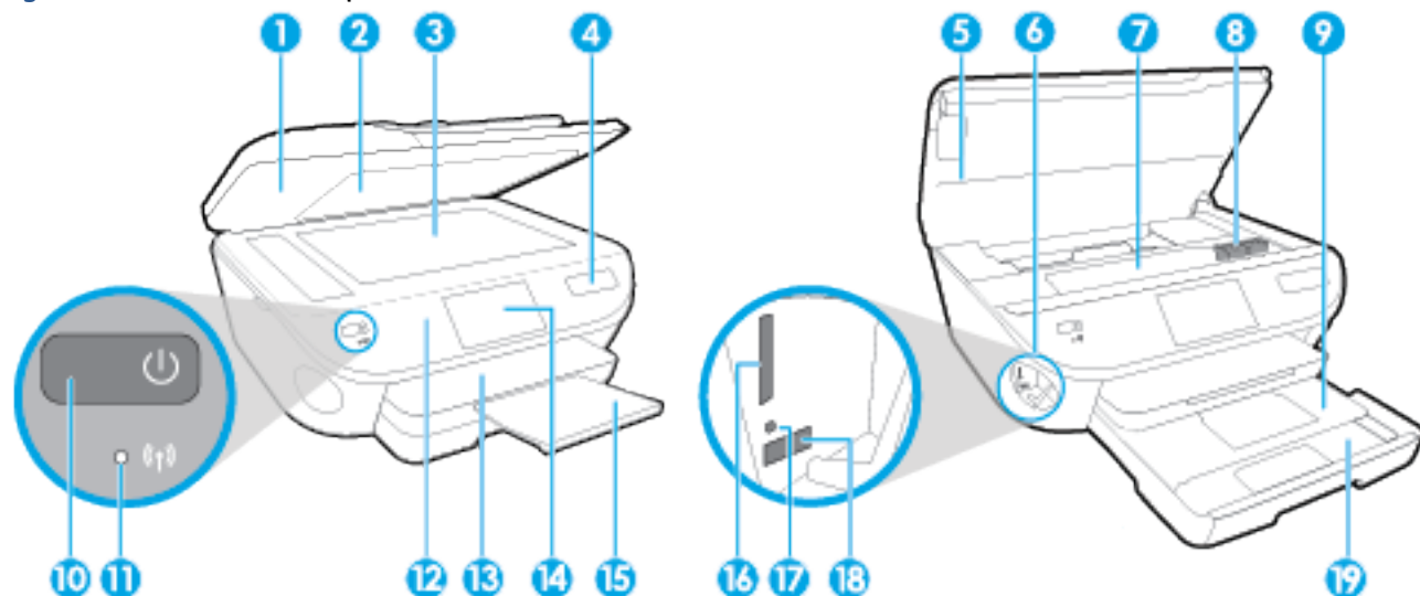
Figura 2-1 Vista frontal e superior do HP ENVY 7640 e-All-in-One series
