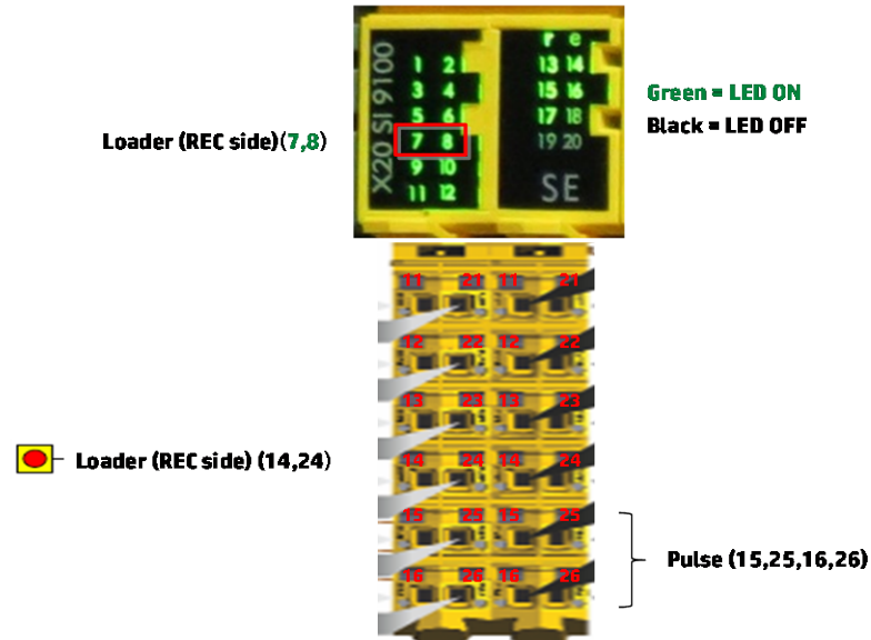
2SD11 LEDs and Connections E.S. Button Loader REC side
