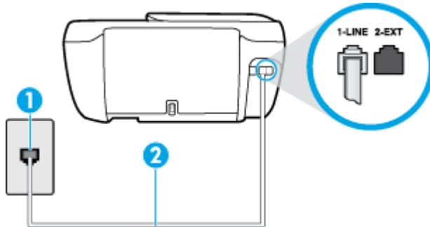
Gambar 9-1 Tampilan belakang printer
