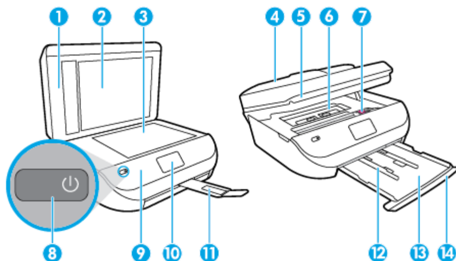
Figura 2-1 Vista frontal e superior do HP OfficeJet 4650 All-in-One series
