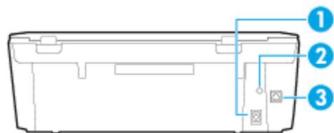
Figure 2-2 Rear view of HP DeskJet Ink Advantage 5640 All-in-One series
