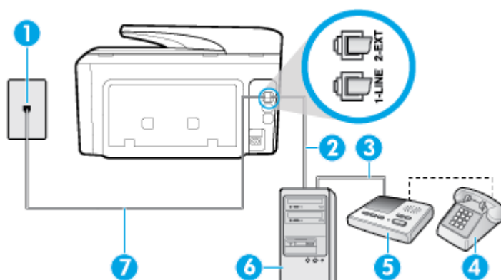
Figur 5-13 Bagsiden af printerens
