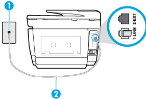
Gambar 5-5 Tampilan belakang printer
