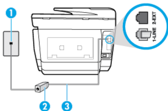
Figur 5-2 Bagsiden af printeren
