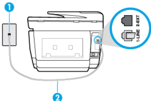
Figur 10-1 Bagsiden af printeren
