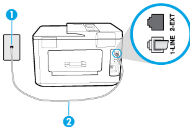
Gambar 5-1 Tampilan belakang printer
