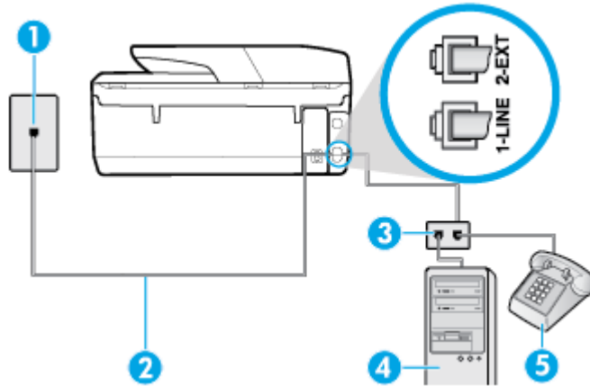
Gambar 5-9 Tampilan belakang printer
