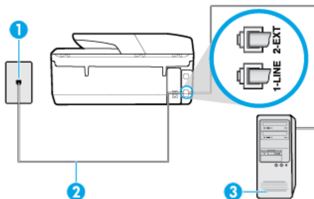
Gambar 5-6 Tampilan belakang printer
