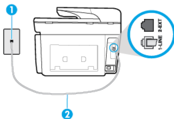
Figur 10-1 Bagsiden af printeren
