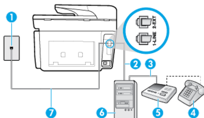
Figur 5-13 Bagsiden af printeren
