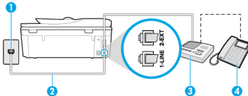
Figure 5-11 Back view of the printer
