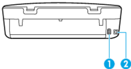
Gambar 2-2 Tampilan belakang HP DeskJet Ink Advantage 5000 All-in-One series
