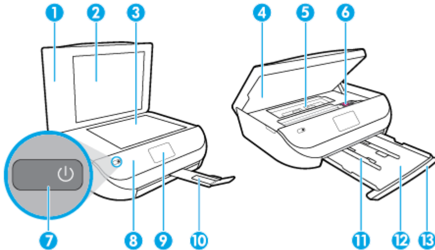
Gambar 2-1 HP DeskJet Ink Advantage 5000 All-in-One series tampak depan dan atas
