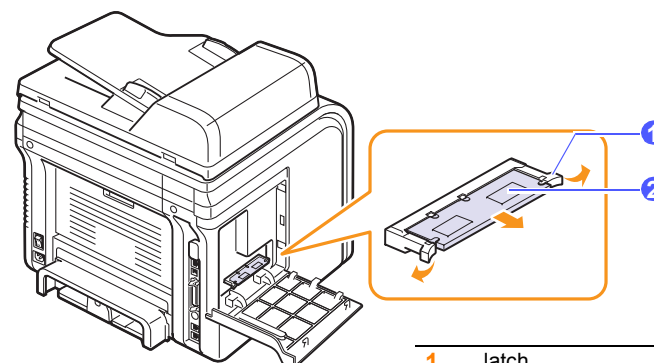
1 latch 2 memory DIMM
