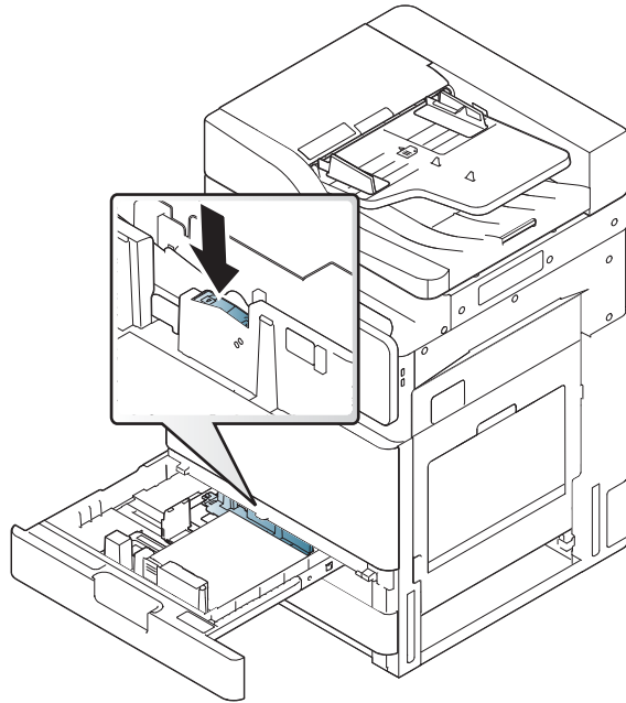
1 Locking switch
