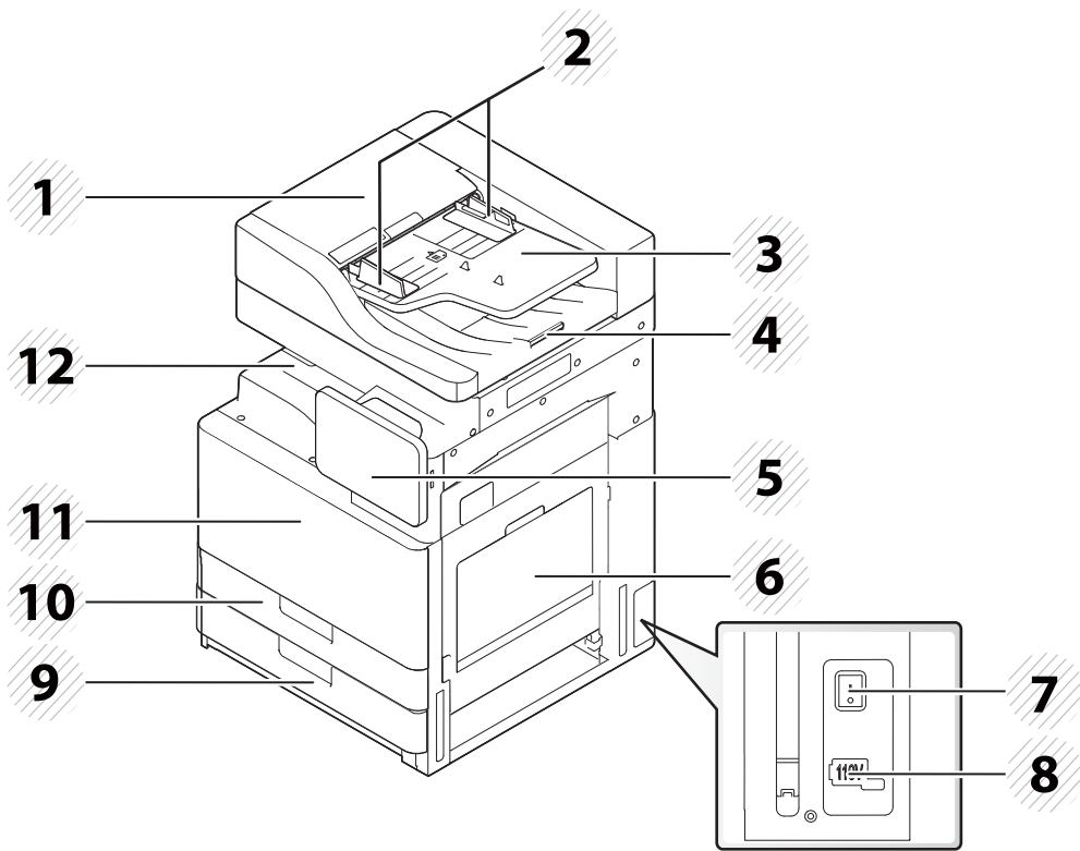
Front view 1
