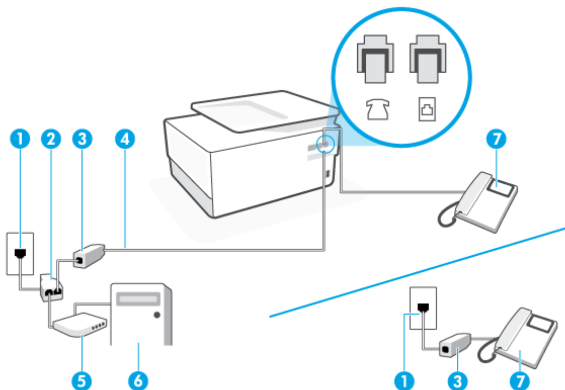
Figur 8-10 Bagsiden af printeren
